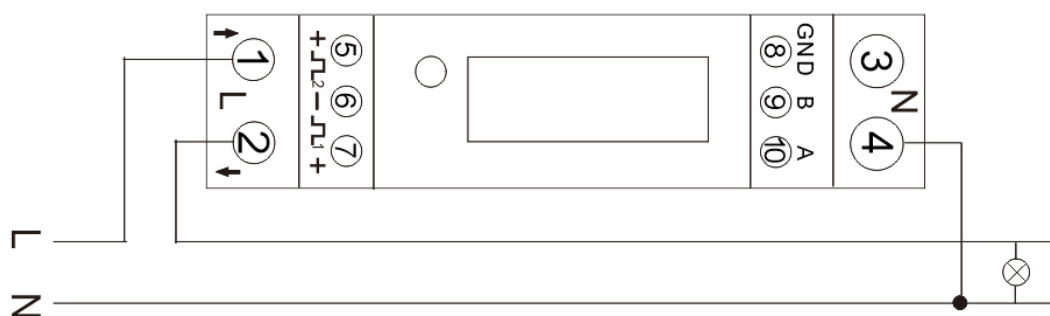
1: L-in 2: L-out 3 / 4: N 5 / 6 / 7: PO 2+ / Com / PO 1+ 8 / 9 / 10: GND/RS485 B/A
