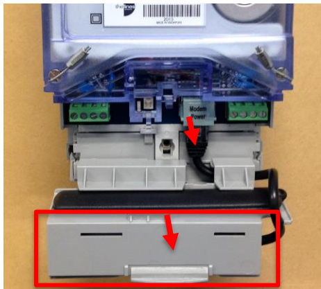
1. Remove modem cover and unplug RJ45
