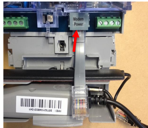
2. Fit short RJ45-RJ45 link cable
