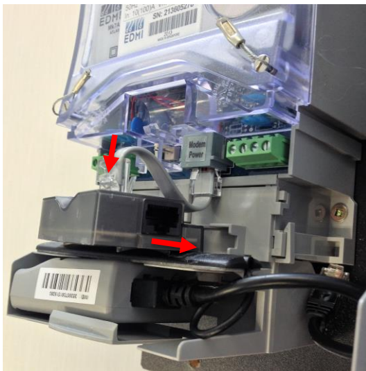
3. Insert Integrator into terminal cover slot and plug in the interconnect cable.
